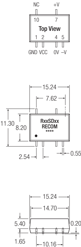
10 Pin SMD Package Style
