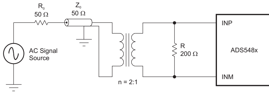
Figure 61. Converting a Single-Ended Input to a Differential Signal Using an RF Transformer
