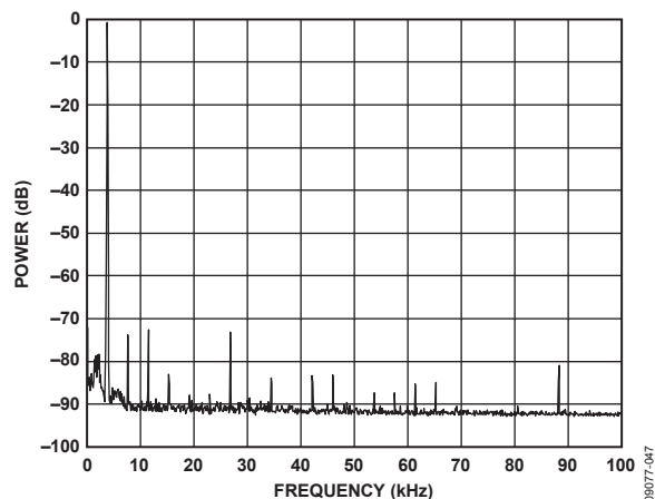
Figure 15. Power vs. Frequency, f_{CLK} = 16 MHz, f_{OUT} = 3.8 kHz, Frequency Word = 0x000FBA9
