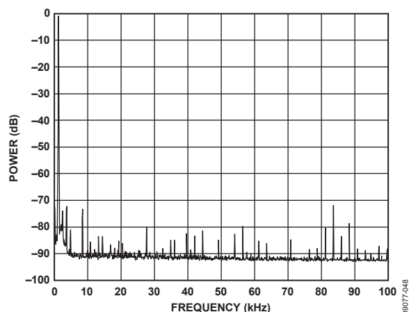
Figure 16. Power vs. Frequency, f_{CLK} = 5 MHz, f_{OUT} = 1.2 kHz, Frequency Word = 0x000FBA9
