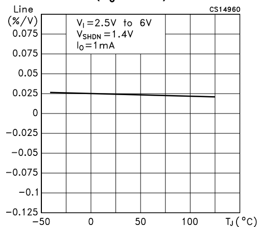
Figure 9. Line regulation vs. temperature ( V_0=1.35\text{ V} )
