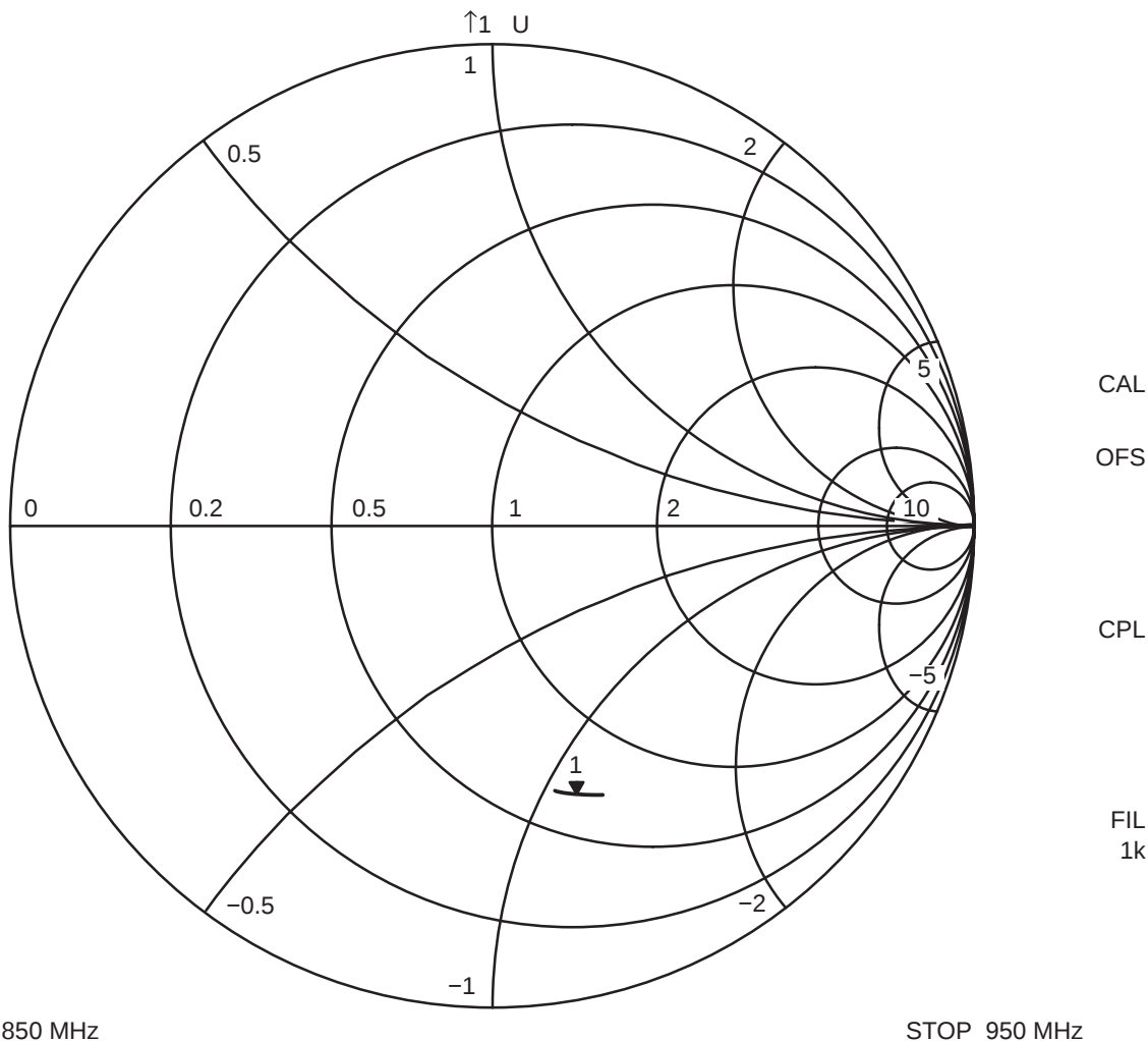
Figure 11. Power Amplifier Output Impedance (S22) at Device Terminal 22
