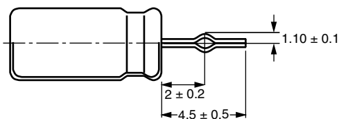
10 \leq \varnothing D \leq 18 leads shortened and formed MALREKS26... (S = 5/7.5 mm)
