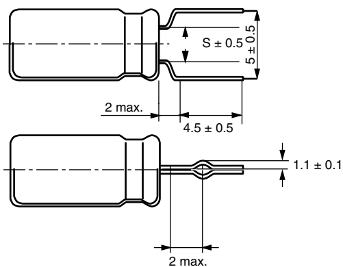
\varnothing D \leq 8 leads shortened and formed MALREKS29... (S = 2.0/2.5/3.5 mm)
