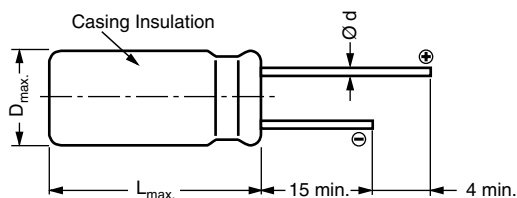
\varnothing D \leq 18 long leads MALREKS20...
