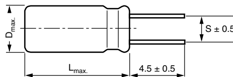
\varnothing D \leq 18 shortened leads MALREKS25... (S = 2/2.5/3.5/5/7.5 mm)
