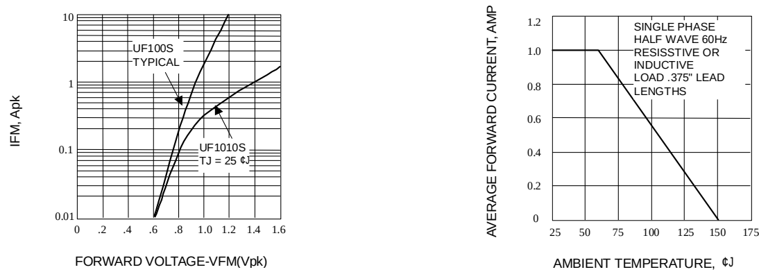
Fig. 2-FORWARD CHARACTERISTICS
