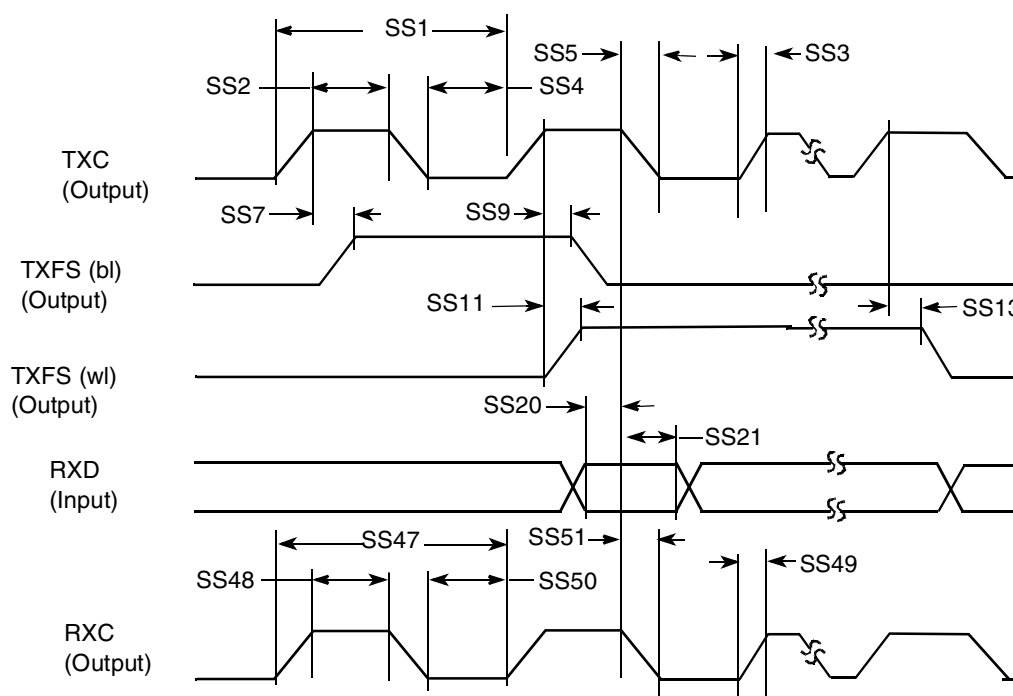
Figure 52. SSI Receiver Internal Clock Timing Diagram
