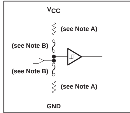
CMOS SCHMITT-TRIGGER INPUT ( \text{CIN} )
