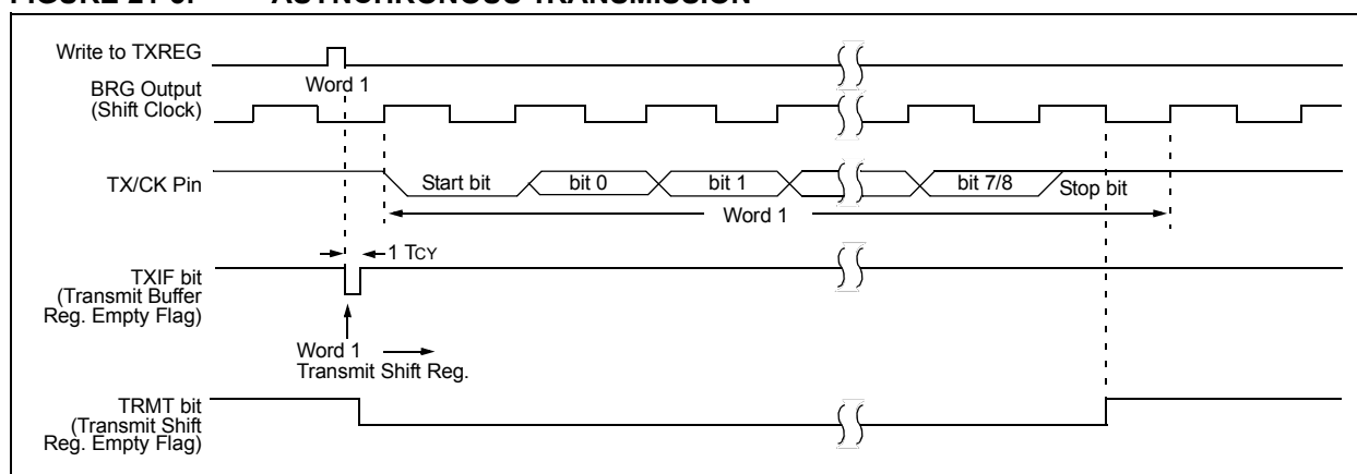
FIGURE 21-3: ASYNCHRONOUS TRANSMISSION
