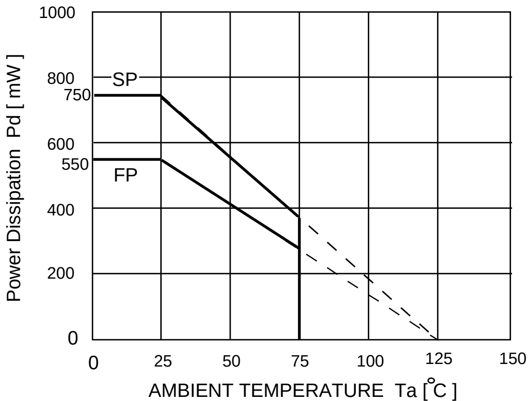
Thermal Derating
