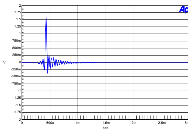
Figure 12. 48 kHz, Impulse Response
