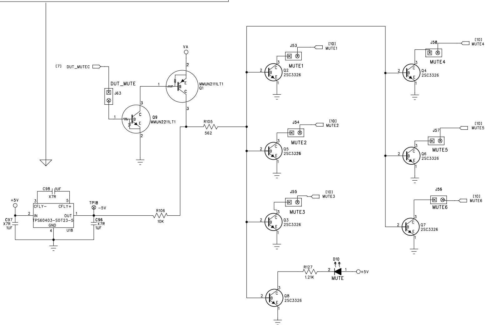
Figure 45. Mute Circuitry
