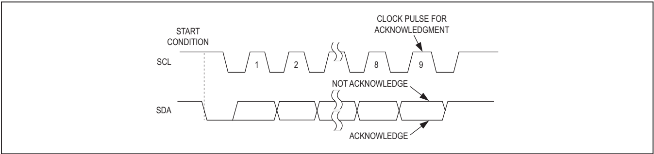
Figure 48. Acknowledge Timing
