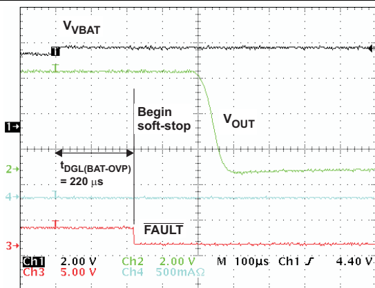
Figure 22. BAT-OVP, V_{BAT} Steps from 4.2\text{ V} to 4.4\text{ V} , Shows t_{DGL(BAT-OVP)} = 220\text{ }\mu\text{s} and Soft-Stop
