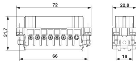
Female insert
