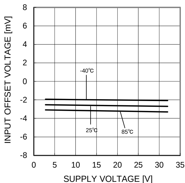
Figure 13. Input Offset Voltage - Supply Voltage (Vcm=0V, OUT=1.4V)
