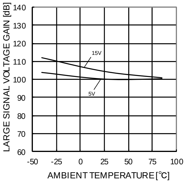
Figure 46. Large Signal Voltage Gain - Ambient Temperature ( R_L=2k\Omega )
