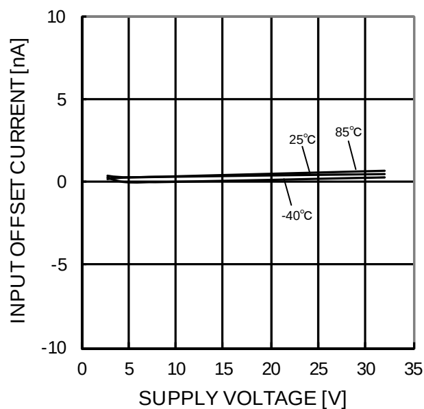
Figure 43. Input Offset Current - Supply Voltage (Vicm=0V, OUT=1.4V)
