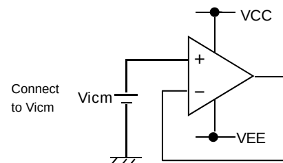
Figure 104. Example of application circuit for unused op-amp
