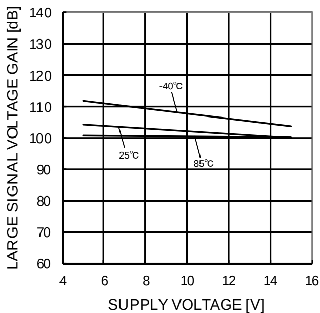
Figure 45. Large Signal Voltage Gain - Supply Voltage (RL=2kΩ)
