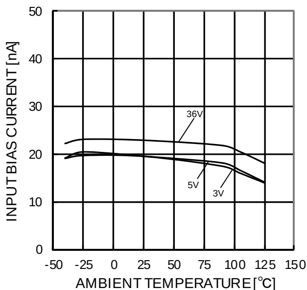
Figure 88. Input Bias Current - Ambient Temperature (Vicm=0V, OUT=1.4V)
