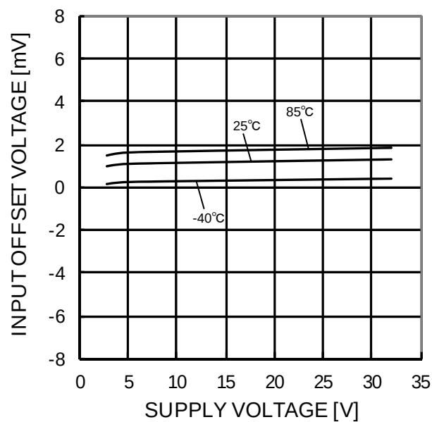
Figure 37. Input Offset Voltage - Supply Voltage (Vcm=0V, OUT=1.4V)
