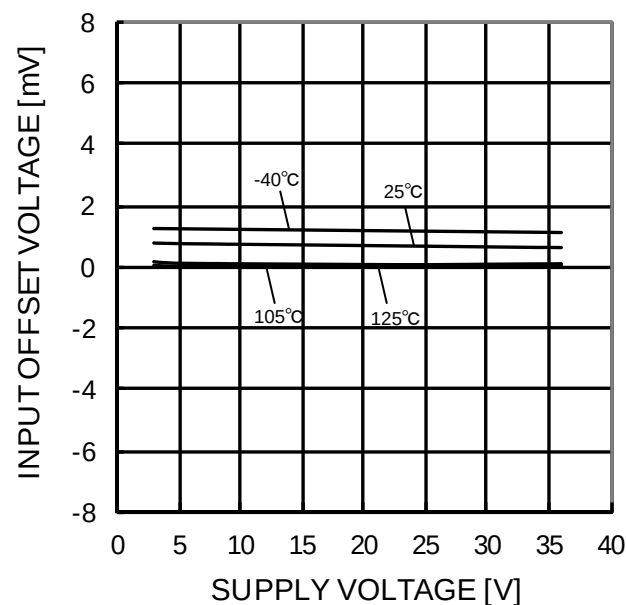
Figure 61. Input Offset Voltage - Supply Voltage (Vcm=0V, OUT=1.4V)
