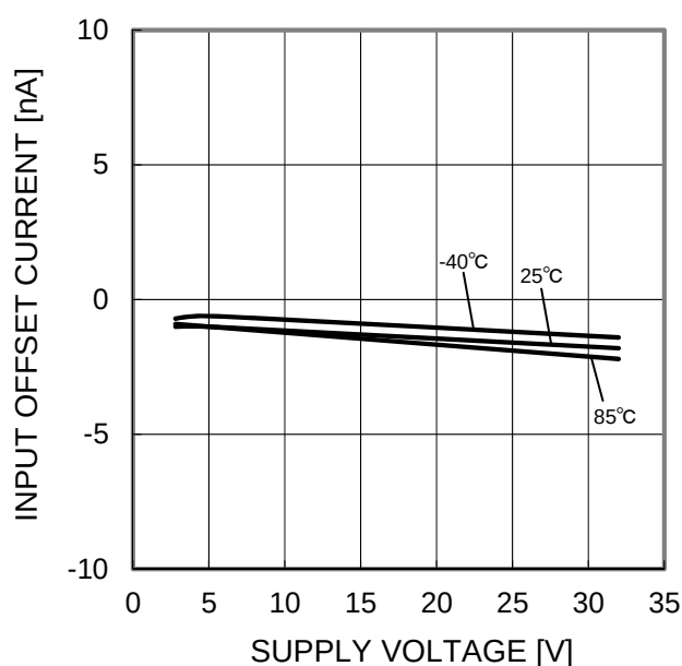
Figure 19. Input Offset Current - Supply Voltage (Vicm=0V, OUT=1.4V)
