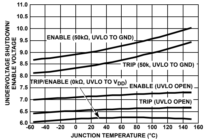
FIGURE 19. UNDERVOLTAGE THRESHOLD
