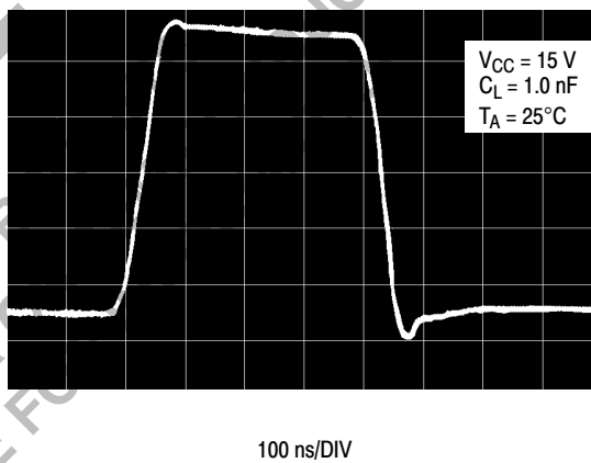
Figure 12. Output Waveform
