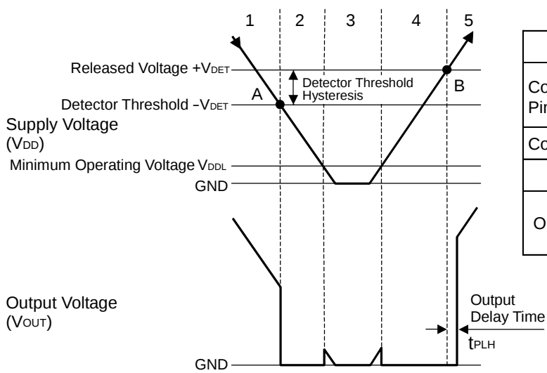
Operation Diagram
