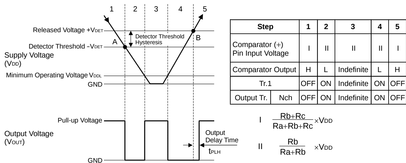
Operation Diagram
