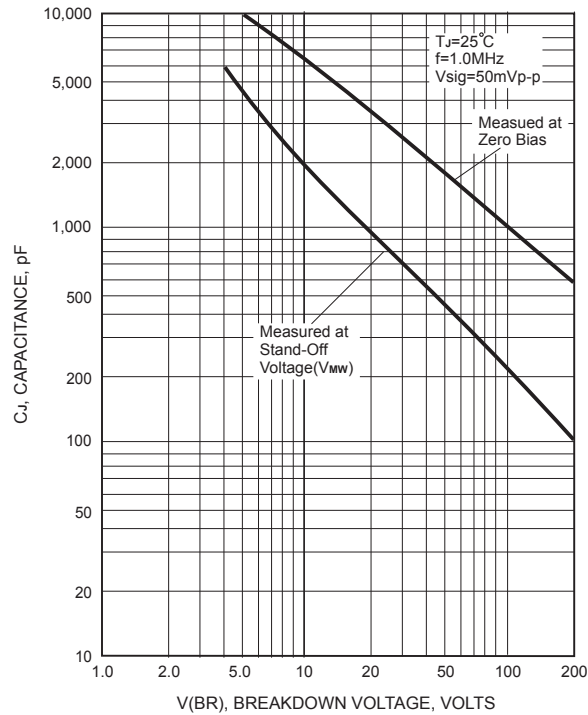
FIG.4-TYPICAL JUNCTION CAPACITANCE
