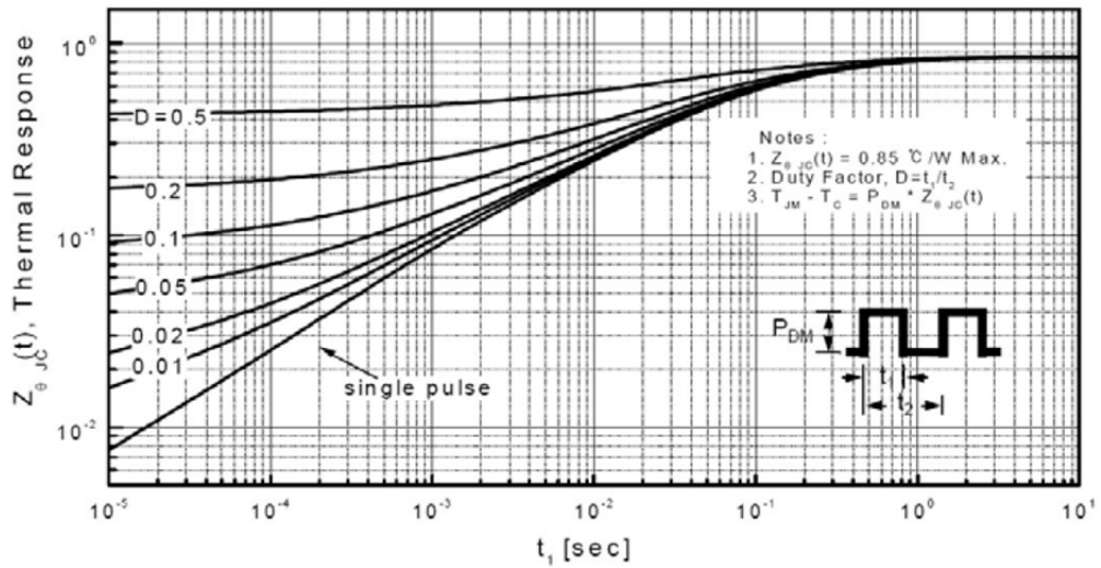
Fig. 9 Transient Thermal Response Curve(TO-220AB)
