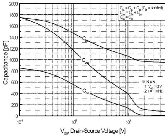
Fig. 5 Capacitance Characteristics
