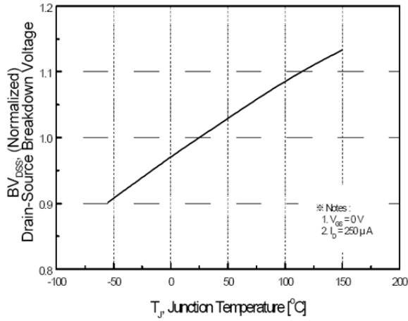
Fig. 3 Breakdown Voltage Variation vs Temperature
