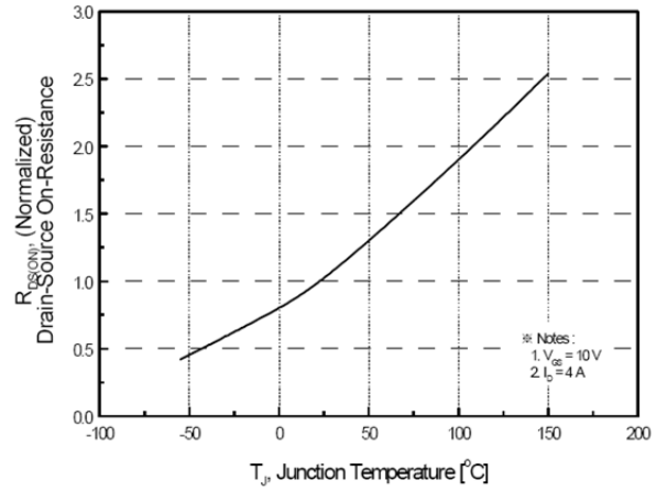
Fig. 4 On-Resistance Variation vs Temperature
