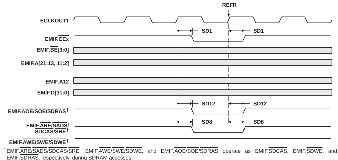
Figure 5–18. SDRAM REFERENCE Command
