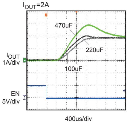
Inrush Current with Different Load Capacitance
