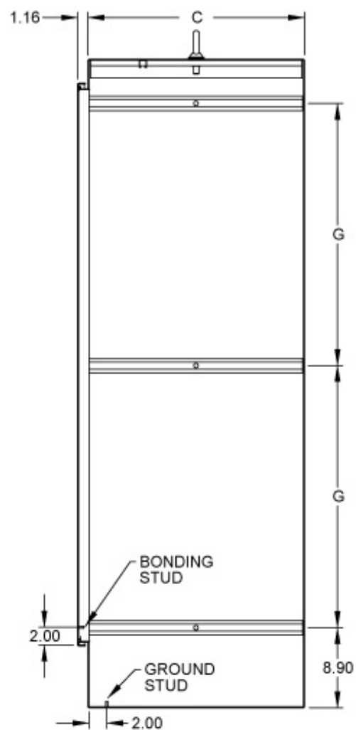
Section Y-Y
