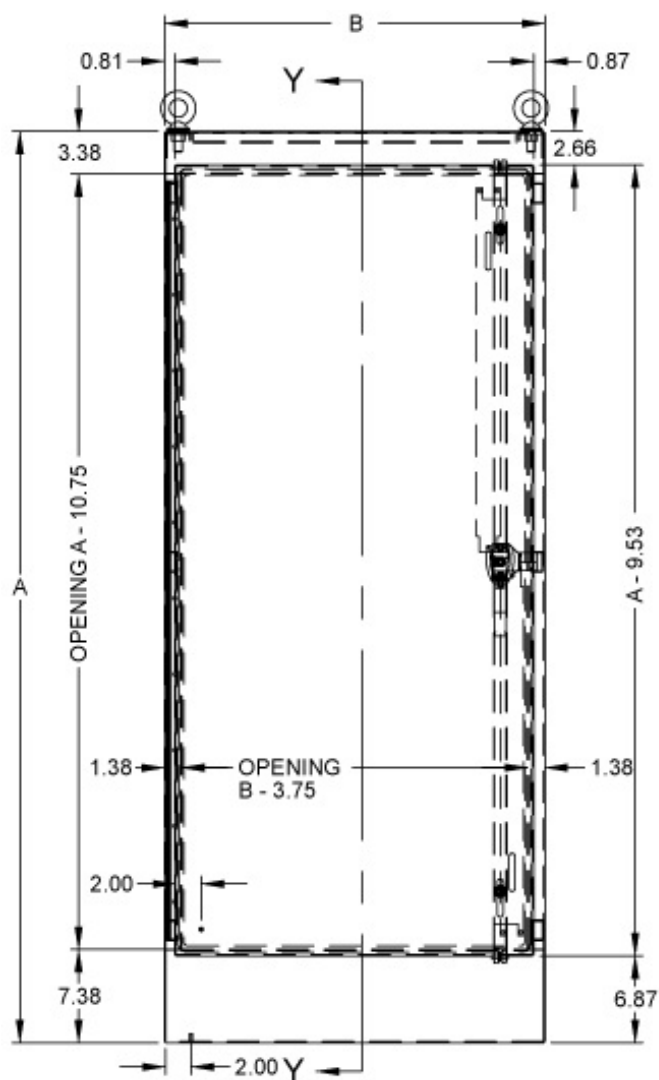
Front View
