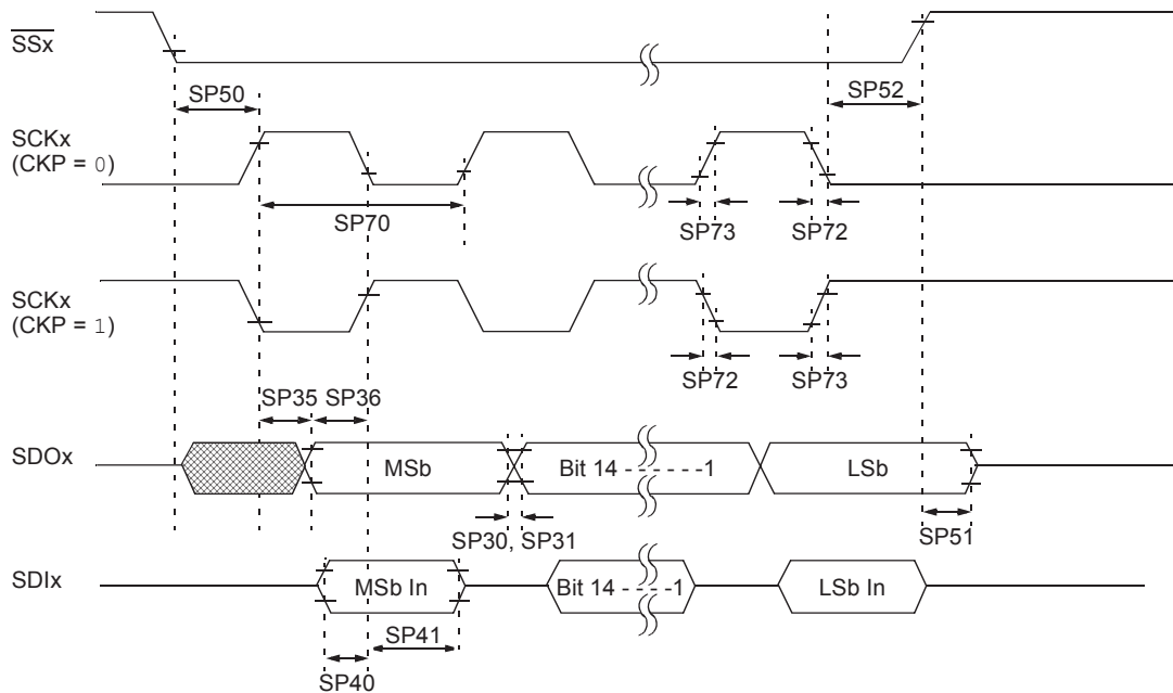
FIGURE 30-17: SPI1, SPI2 AND SPI3 SLAVE MODE (FULL-DUPLEX, CKE = 0, CKP = 1, SMP = 0) TIMING CHARACTERISTICS (1,2)
