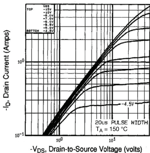
Fig. 2 - Typical Output Characteristics, T_A = 150^\circ\text{C}
