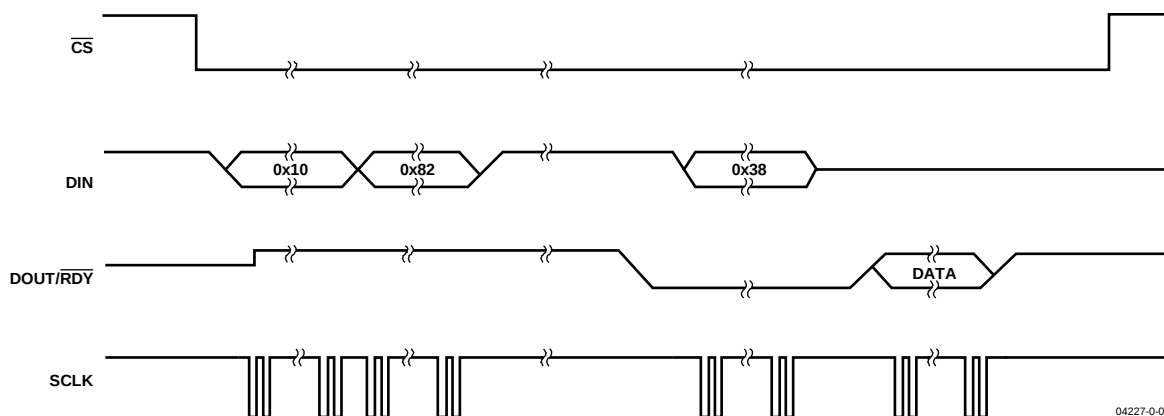
Figure 13. Single Conversion
