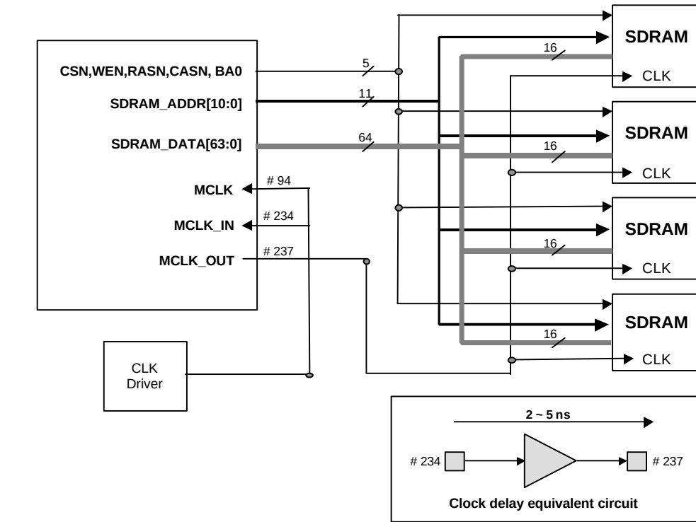
Figure 11. External Memory Interface 2
