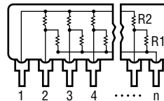
-5 Circuit Dual Terminator
