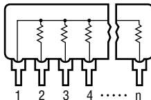
-1 Circuit Bussed Resistors
