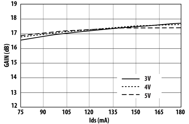
Figure 10. Small Signal Gain vs. I_{ds} and V_{ds} at 900 MHz
