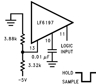
FIGURE 7. ECL Logic
