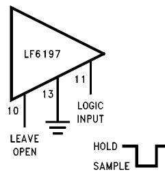
FIGURE 4. TTL Logic
