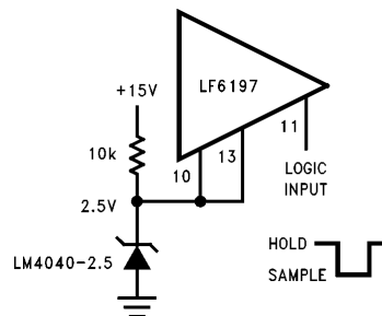
FIGURE 5. CMOS Logic
