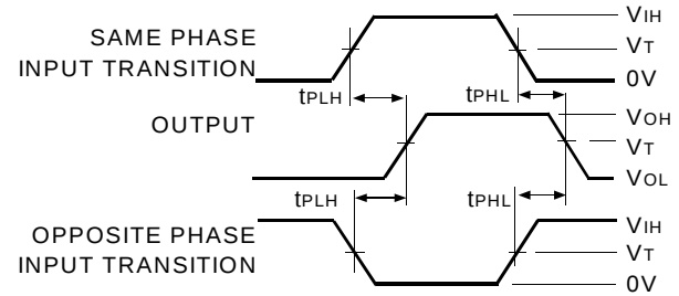
Propagation Delay
