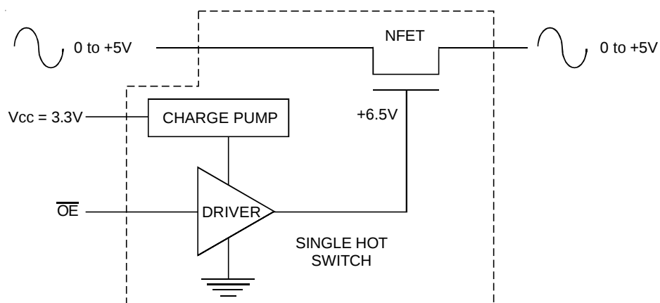
Rail-to-Rail Switching
