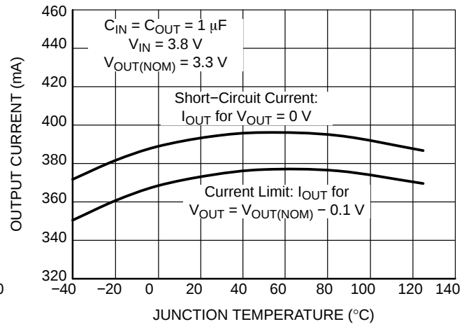
Figure 29. Short-Circuit Limit vs. Temperature V_{OUT} = 3.3\text{ V}
