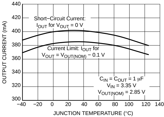
Figure 26. Short-Circuit Limit vs. Temperature V_{OUT} = 2.85\text{ V}
