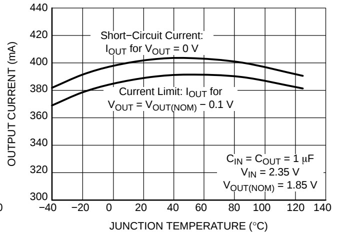
Figure 25. Short-Circuit Limit vs. Temperature V_{OUT} = 1.85\text{ V}
