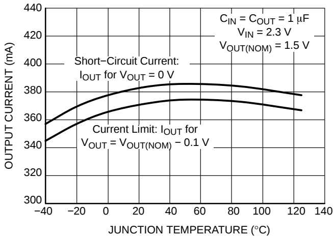
Figure 24. Short-Circuit Limit vs. Temperature V_{OUT} = 1.5\text{ V}
