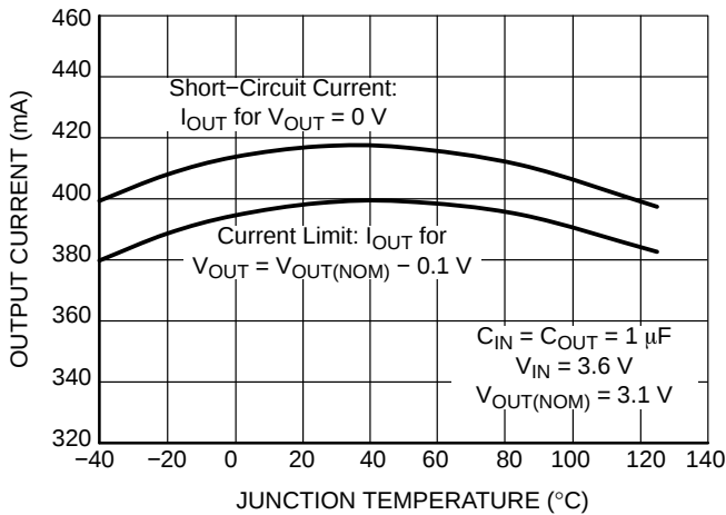
Figure 28. Short-Circuit Limit vs. Temperature V_{OUT} = 3.1\text{ V}
