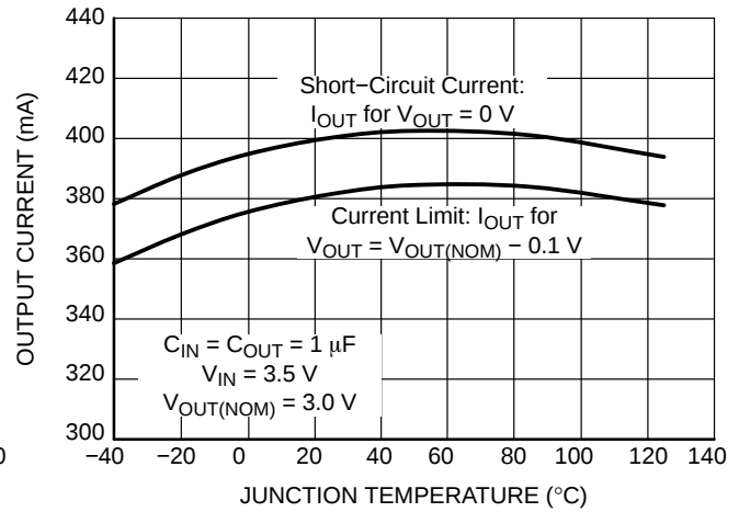
Figure 27. Short-Circuit Limit vs. Temperature V_{OUT} = 3.0\text{ V}
