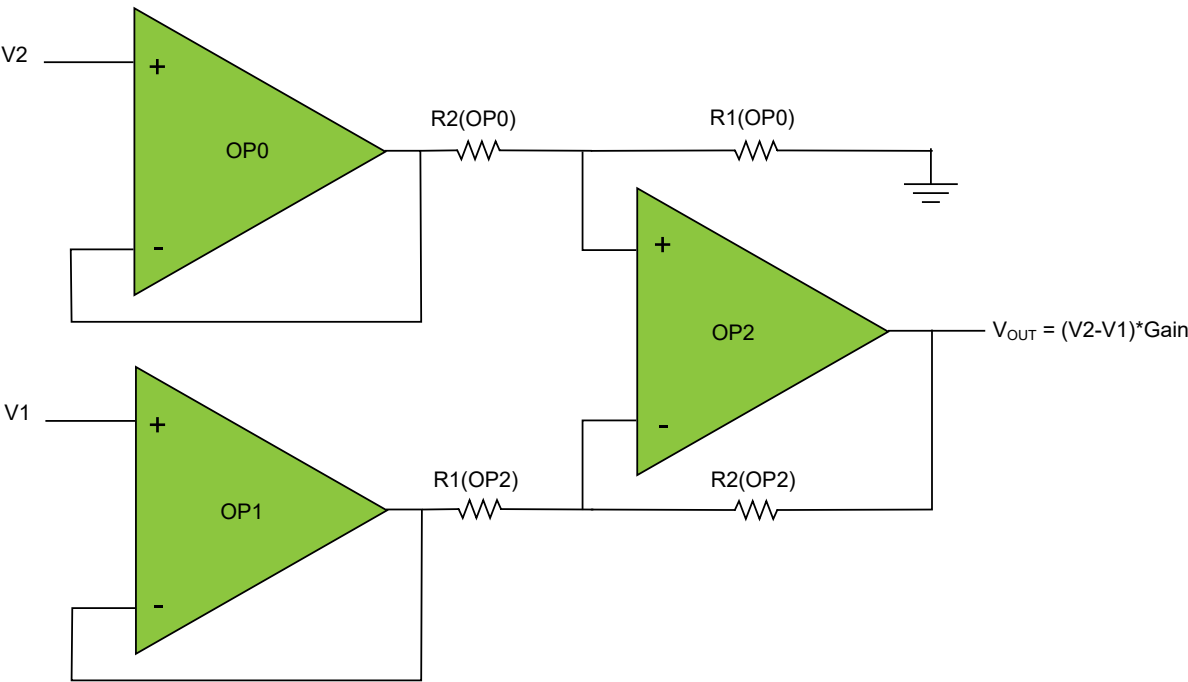
Figure 35-12. Instrumentation Amplifier
