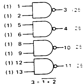
MC857/MC957 Quad 2-Input Buffers
