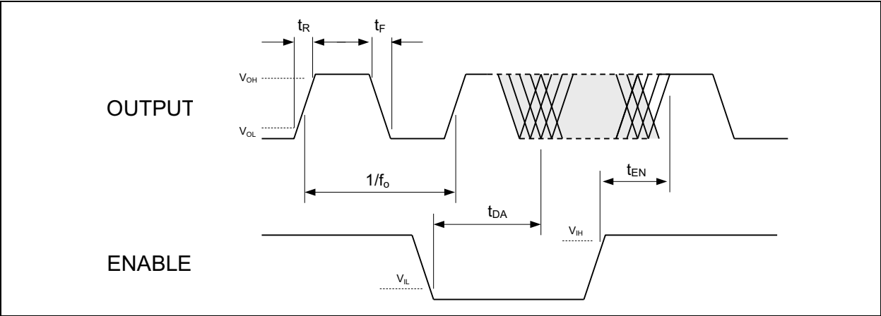
FIGURE 3-1: Output Waveform.
