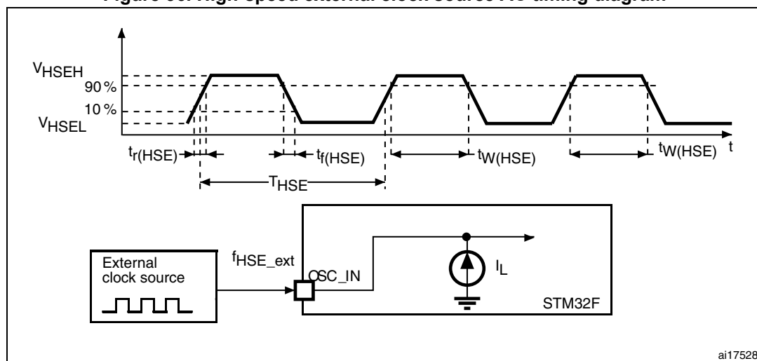
Figure 36. High-speed external clock source AC timing diagram
