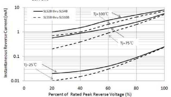
Figure 4. Typical Reverse Characteristics rev.1
