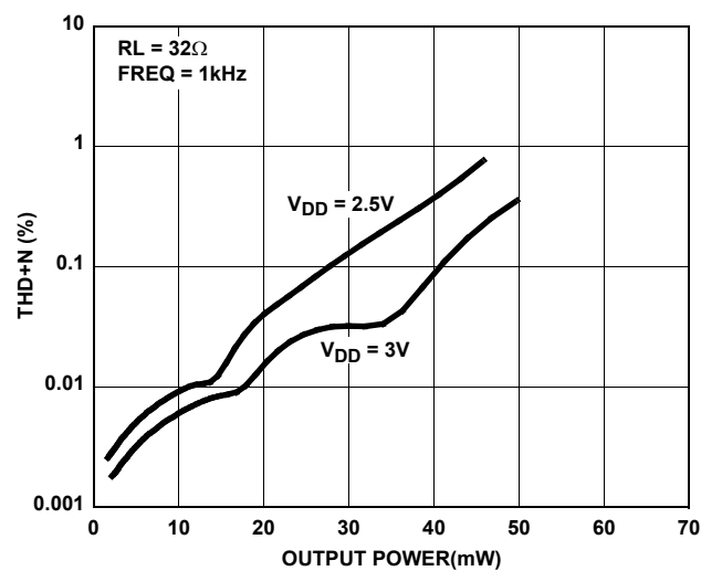
FIGURE 11. THD+N vs POWER
