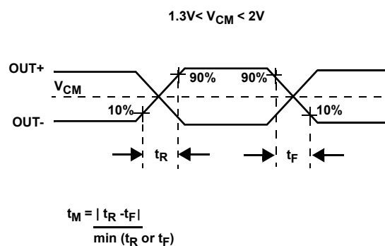
FIGURE 6. RISE/FALL TIME MISMATCH TEST
