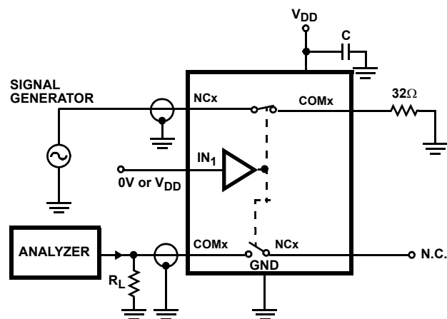
FIGURE 2. BREAK-BEFORE-MAKE TIME (ISL54417 ONLY)
