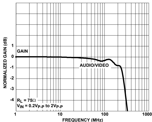
FIGURE 14. FREQUENCY RESPONSE
