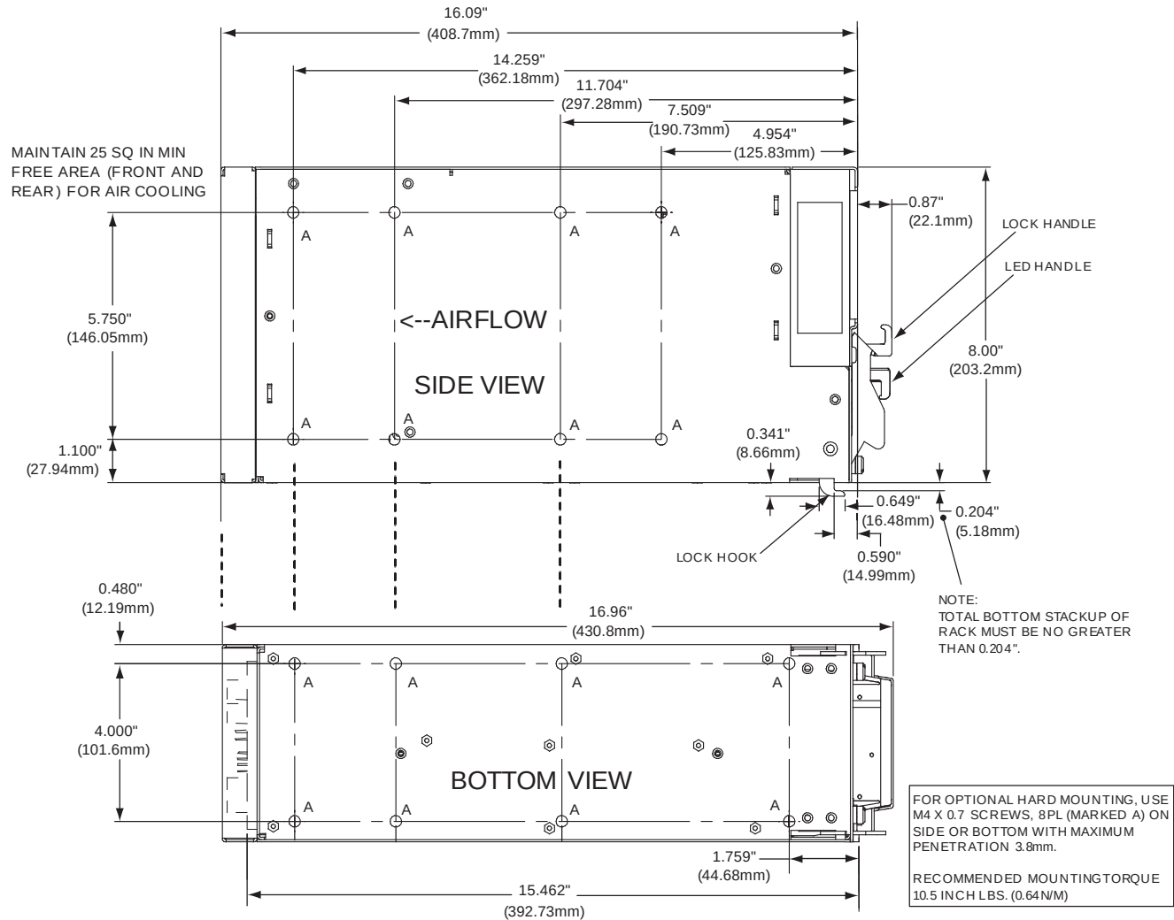
Figure 2 – FXP7000 Overall Size
