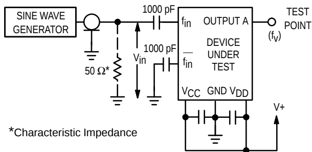
Figure 7. Test Circuit
