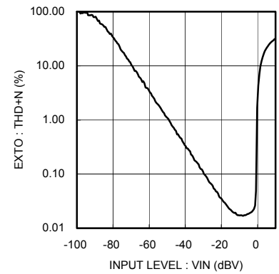
Fig.6 Total Harmonic Distortion (EXTO)
