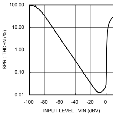
Fig.8 Total Harmonic Distortion (SPR)
