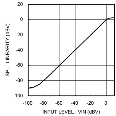
Fig.12 Linearity (SPL)
