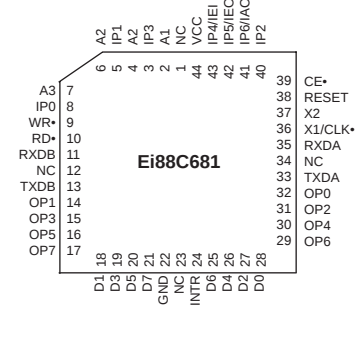
44-PIN PLCC
