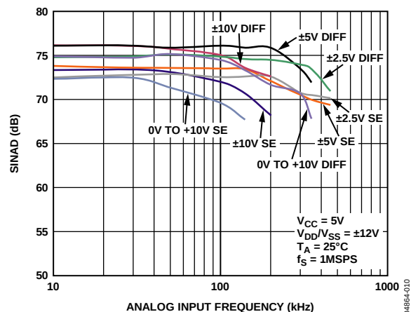
Figure 12. SINAD vs. Analog Input Frequency for Single-Ended (SE) and True Differential Mode (Diff) at 5 V_{CC}
