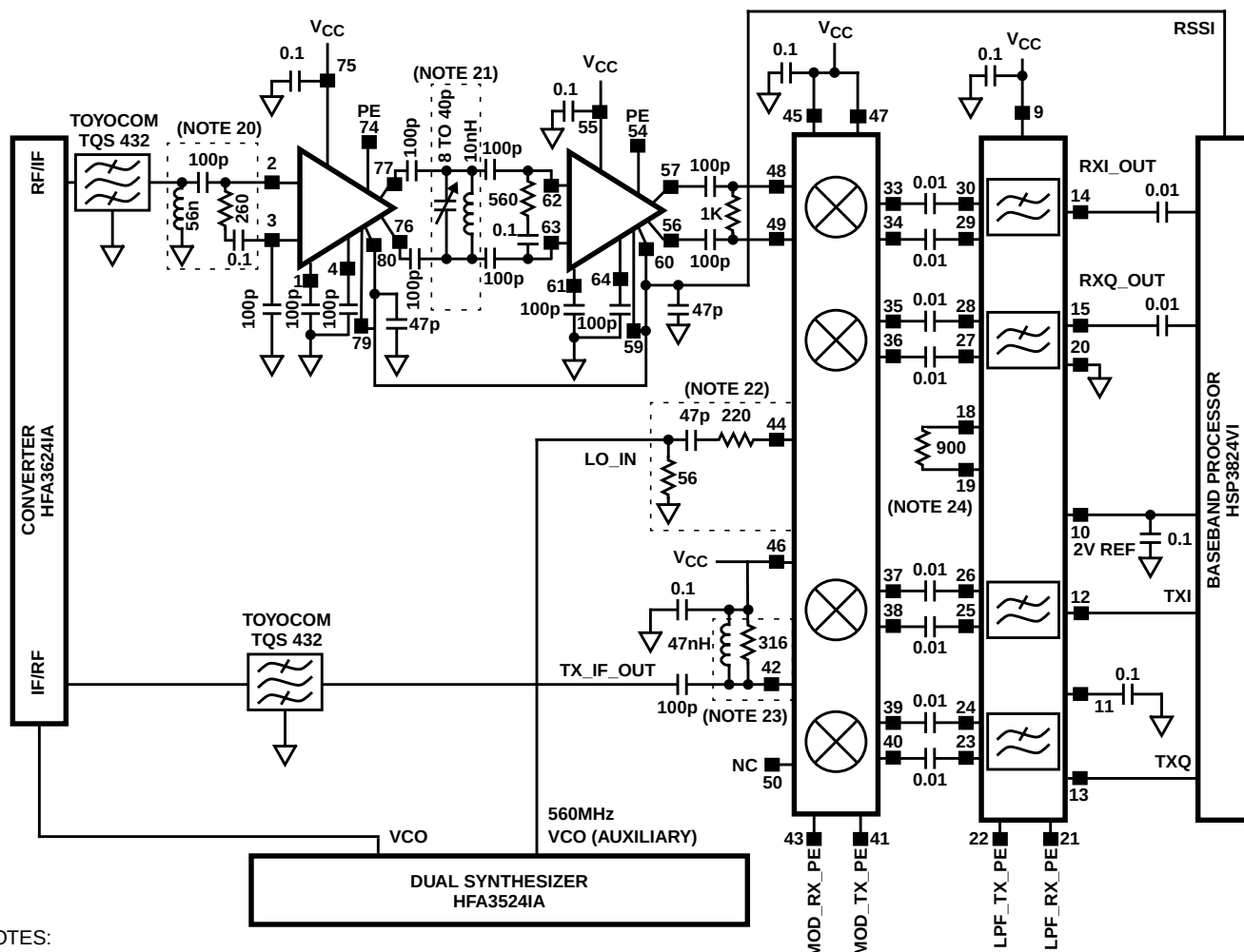
Typical Application Diagram (Targeting IEEE 802.11 Standard)
