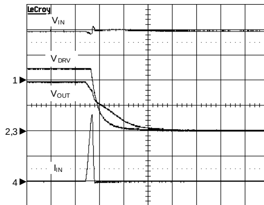
Short Circuit After Power On
