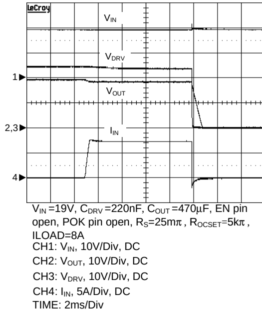
OCP and Its Debounce Time
