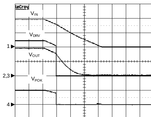
Power Off with POK Pulled High
