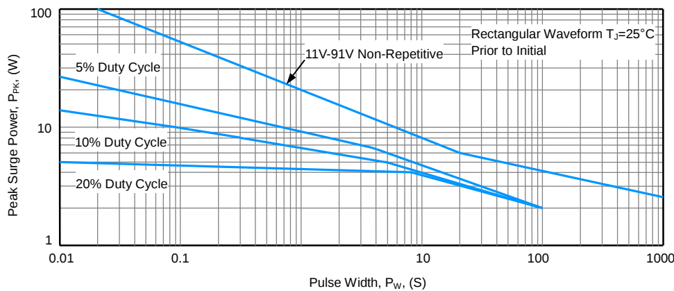
Figure 4 - Maximum Surge Power
