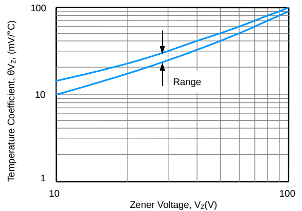
Figure 2 - Temperature Coefficients v.s. Zener Voltage
