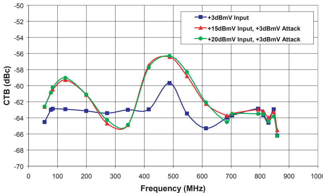
Figure 7: CTB vs. Frequency (129 channels - flat, T_c = +55^\circ\text{C} )
