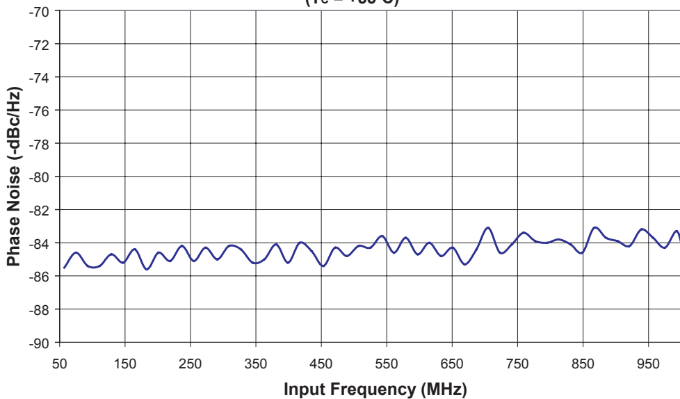
Figure 10: Composite Oscillator Phase Noise @ 10 KHz Offset ( T_c = +55^\circ\text{C} )
