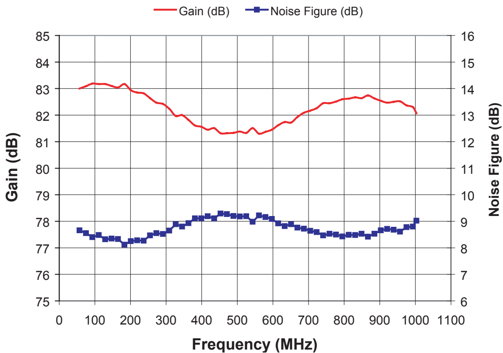
Figure 9: Gain & NF vs. Frequency ( T_c = +55^\circ\text{C} )
