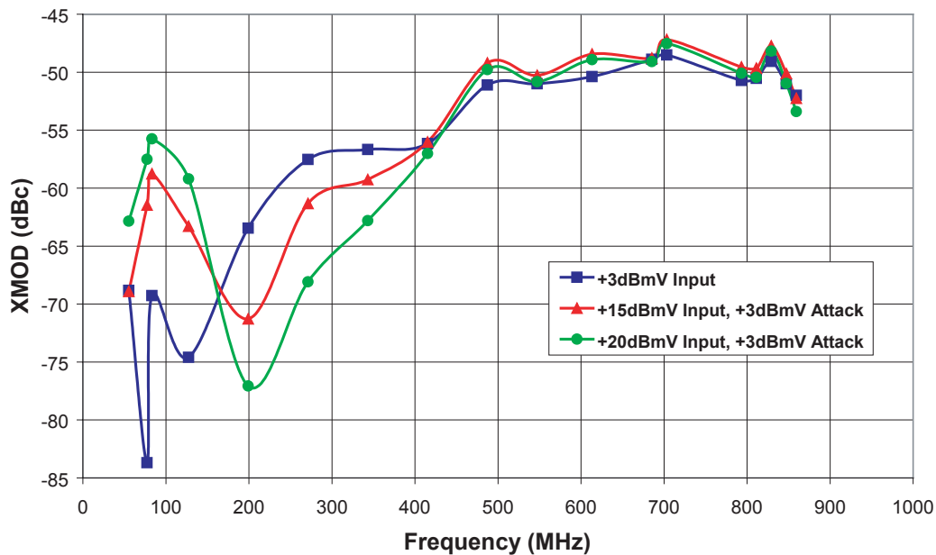
Figure 8: XMOD vs. Frequency (129 channels - flat, T_c = +55^\circ\text{C} )
