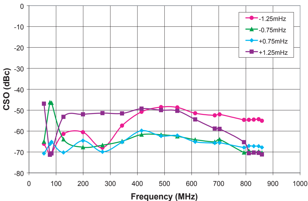
Figure 5: CSO vs. Frequency (+15 dBmV input power, +3dBmV Attack, 129 channels - flat, T_c = +55^\circ\text{C} )
