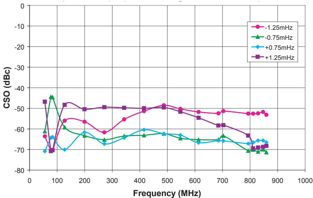
Figure 4: CSO vs. Frequency (+3dBmV input power, 129 channels - flat, T_c = +55^\circ\text{C} )
