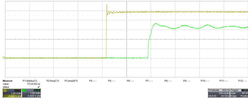
Figure 22. t_LOOP Delay
