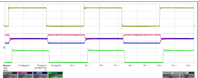
Figure 24. HVDA540 TXD, CANH, CANL and RXD Waveforms at 500 Kbps
