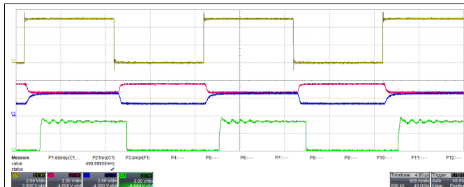
Figure 23. HVDA540 TXD, CANH, CANL and RXD Waveforms at 1 Mbps
