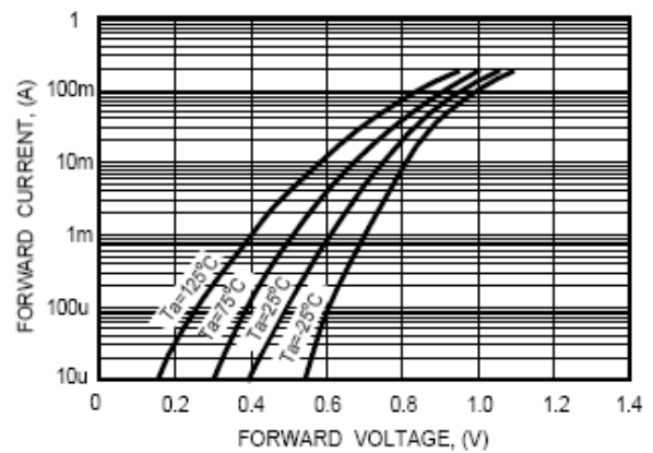
FIG. 2 - FORWARD CHARACTERISTICS
